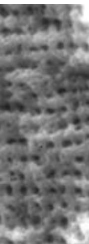
THREE-DIMENSIONAL LATTICE of liquid-crystal droplets [etched away for this micrograph] forms a photonic crystal whose properties can be controlled by applying a voltage. The holes are each separated by about 0.25 micron.
